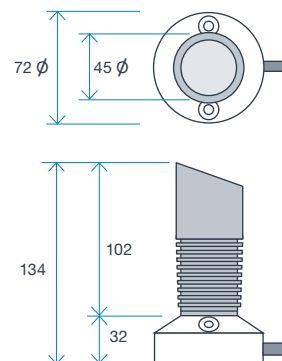
Mount fixing
